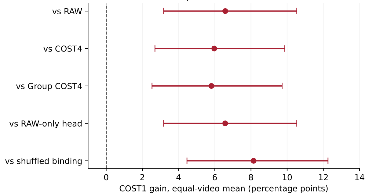
95% bootstrap intervals: 27 source videos
